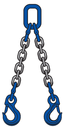
2 LEG SLING
